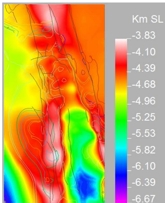
Figure 5: Derived 2D grid of depth to the 150°C isotherm (from the 3D voxel of temperatures), together with a colour legend for depth. The image is geo-located in the surface geology section to show the locations of fault traces (grey lines) and upper geology boundaries (colour legend from Fig. 1).
