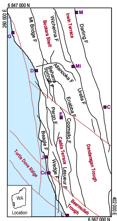
Figure 2: Location, structural elements and fault trace map of the north Perth Basin, Western Australia. [M= Mullewa; G=Geraldton; Mi=Mingenew; D=Dongara; C=Carnamah; E=Eneabba; J=Jurien; Ce=Cervantes; L=Lancelin.]
