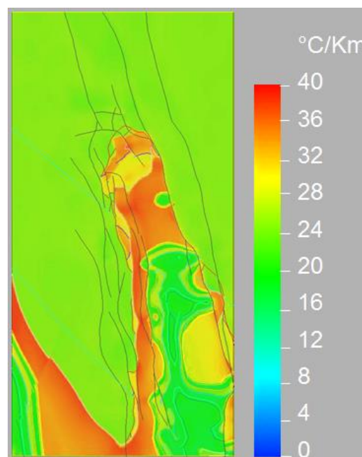
Figure 7: Modelled vertical temperature gradients ( ^{\circ}\text{C}/\text{Km} ) for the -4000m below SL section. The image is geo-located in the matching horizontal section of the geology model to show the locations of faults (grey lines) and geology boundaries.
