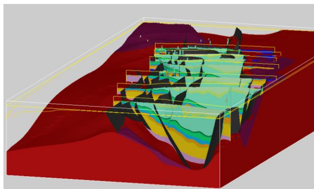
Figure 3: Oblique 3D view of the northern Perth Basin (from the south-east). Vertical exaggregation 3:1. This composite model presents solid volumes of Pre-Cambrian basement gneisses, rendered 2D sections of the Permian to Late Cretaceous basin sequences, modelled fault surfaces and exaggerated views of well intercepts (well radii 350m).
