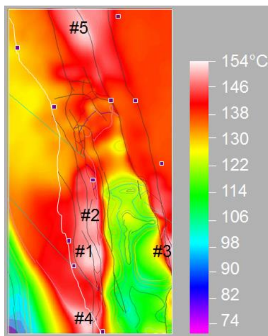
Figure 4: Plan view of computed 3D temperatures sliced through the -4000m level, together with the colour legend for the derived 2D grid (linear stretch). Locations of 5 high temperature anomalies (Table 4) are shown together with locations of faults and upper geology boundaries. Squares = town-locations from Fig. 1.
