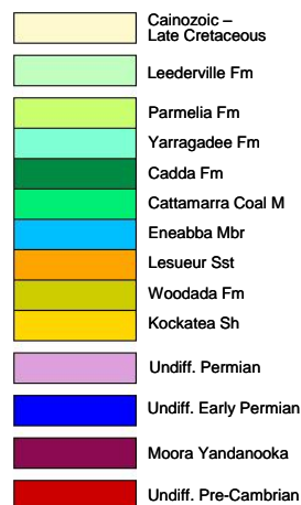
Figure 1: Stratigraphy of the north Perth Basin used to build the geology model. Note grouped units of the basin-fill are modeled with a single interpolator, while each unit separate within the pile, is modeled with an independent interpolator.
