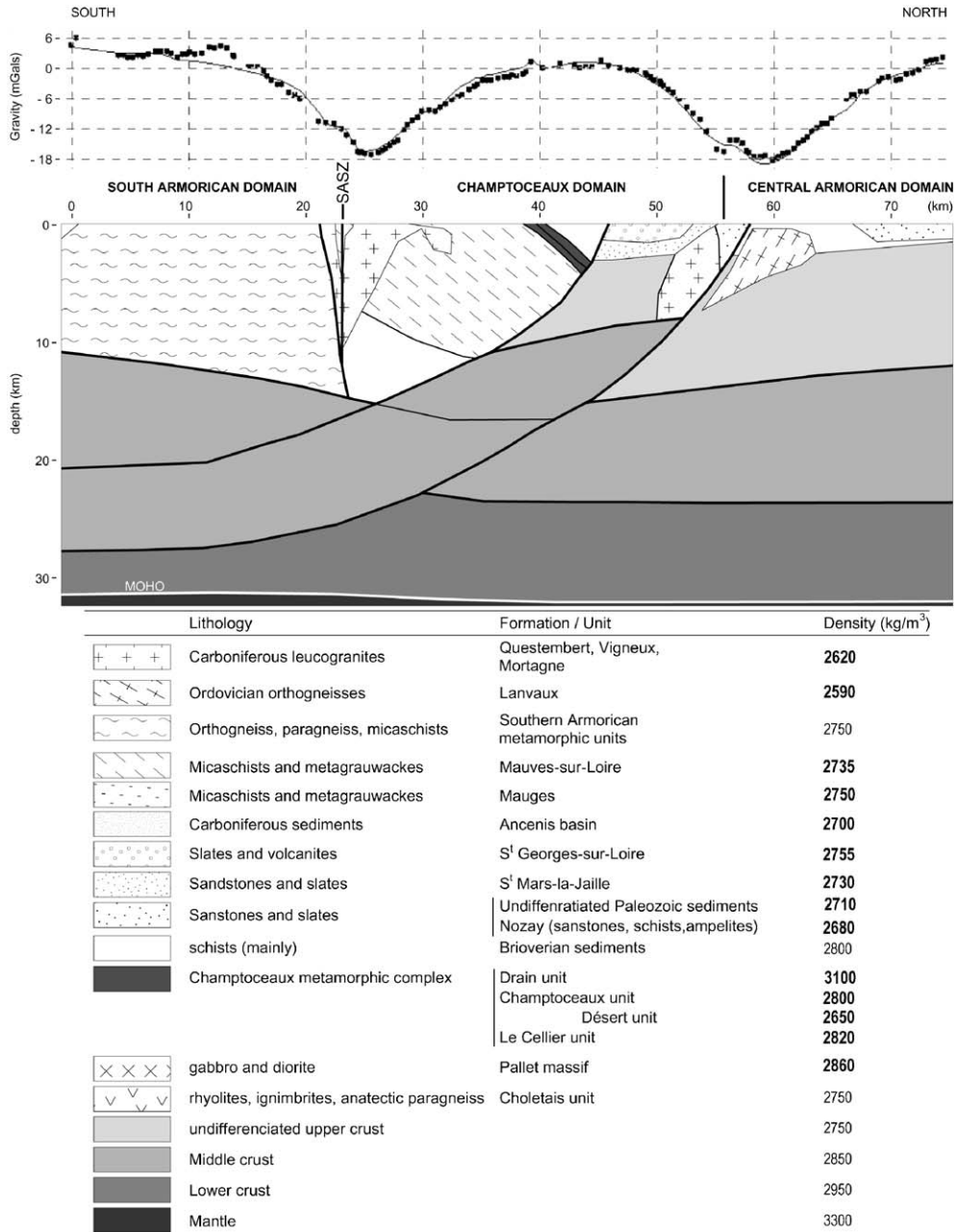
Fig. 4. Direct 2D gravity modelling along profile 3 (see location on Fig. 3). The interpretation of Armor 2 seismic section (black thick lines) constrains the geometry of mid to lower crust units. The model gravity effect (thin black curve on upper window) has been fitted to Bouguer anomaly data (black dots on upper window) using surface geology (lithologies and structural data) and available shallow seismic reflections. A good fit of the central midwavelength-positive anomaly necessitates the occurrence of a dense body underneath the Champtoceaux complex. A possible candidate can be a relative uplift of middle crust along the crustal-scale south dipping shear zone system deduced from seismics (see Fig. 2). The different units (symbols as on Figs. 1 and 2) and corresponding densities used in the modelling are listed (sample or well-logging density measurements are in bold).
