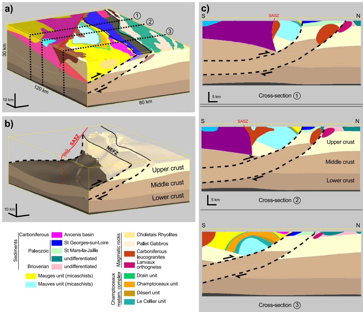
Fig. 7. (a) View from the SE of the 3D block modelled in Champtoceaux area, with location of the three cross-sections shown in (c). The south dipping crustal-scale shear zone is highlighted by black dotted lines. (b) View of the middle to lower crustal interfaces beneath the Champtoceaux complex after removal of more superficial units. The south dipping crustal-scale shear zone becomes subvertical at the vicinity of the SASZ (in red). (c) Extraction of three parallel cross-sections from the 3D model, outlining the evolution of the Champtoceaux Domain from west to east. To the south, this Domain is sheared along the SASZ, and to the north, it is folded (orange and blue in cross-section 3) above the crustal-scale shear zone. The three cross-sections also illustrate the elongate shape of granitic bodies (Questembert and Lanvaux) that extend in subsurface, perpendicular to the cross-sections, along the south dipping wrench–thrust system.
