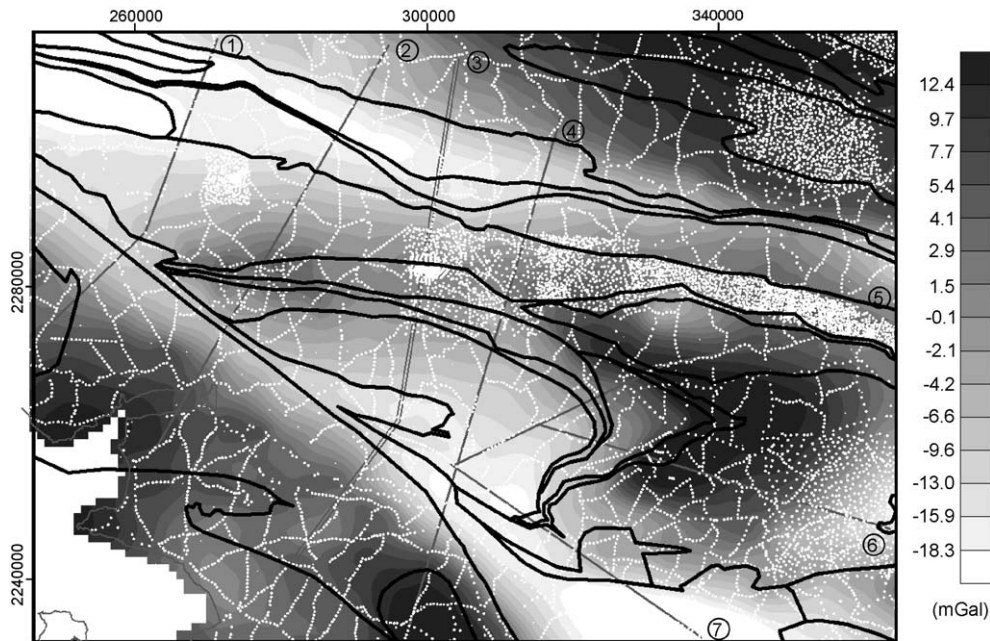
Fig. 3. Bouguer anomaly map in the Champtoceaux area (see location on Fig. 1). White dots are locations of available gravity data. Black thin lines indicate locations of the seven gravity cross-sections used in the modelling. Profile 3 coincides with the Armor 2 seismic profile (Fig. 2). Black thick lines correspond to simplified geological contours used for modelling.
