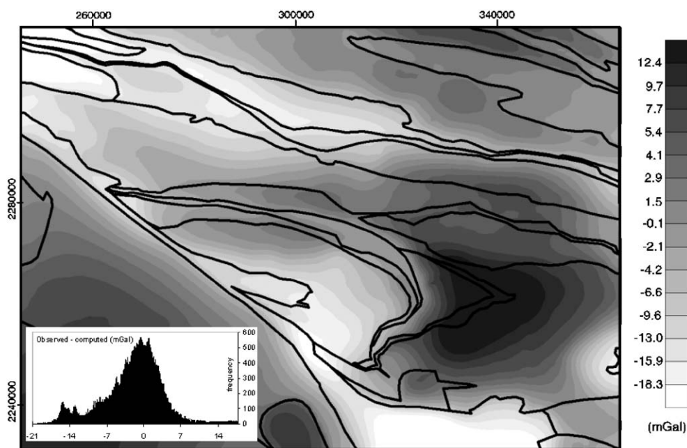
Fig. 5. Computed 3D gravity effect of the 3D model, using densities reported in Fig. 4. A good consistency is obtained between this model gravity map and the Bouguer anomaly map (Fig. 3), which is confirmed by the discrepancy histogram. In particular, middle- to short-wavelength anomalies located between the two branches of the SASZ fit the measured anomaly fairly well.
