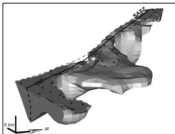
Fig. 6. 3D view from the SE of the leucogranites which have been sheared along the southern branch of the SASZ. Black dotted lines show the outcropping limits of granites. The shape of the Vigneux granite (centre of the figure) clearly exhibits its laccolithic nature.
