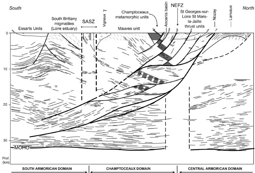
Fig. 2. Interpretation of the Armor 2 seismic profile (located on Fig. 1) (modified after Bitri et al., 2003). Major interpreted structures are highlighted by black lines; less constrained structures and interruptions of reflections are underlined by dotted lines. SASZ, South Armorican Shear Zone; NEFZ, Nort-sur-Edre Fault Zone. Surface geological units as on Fig. 1. See text for detailed description.
