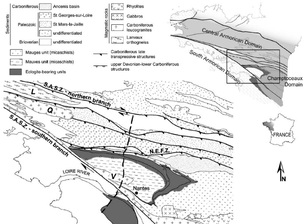
Fig. 1. Simplified geological map of the Champtoceaux area in the Hercynian belt of Brittany. SASZ, South Armorian Shear Zone; NEFZ, Nort-sur-Erdre Fault Zone; Q, Questembert granite; L, Lanvaux orthogneiss; V, Vigneux granite. Black rectangle shows limits of the 3D modelling area; thick dashed line is the location of the Armor 2 seismic profile (Fig. 2).
