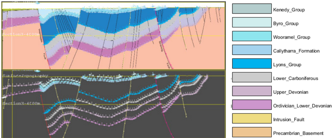
Figure 6 - Upper: Interpreted seismic section (after Iasky et al., 1998) which was geolocated in GeoModeller, and used to digitize geological constraints (Lower) for the initial 3D geology model. Right: Stratigraphic pile for the Merlinleigh Sub-basin.
