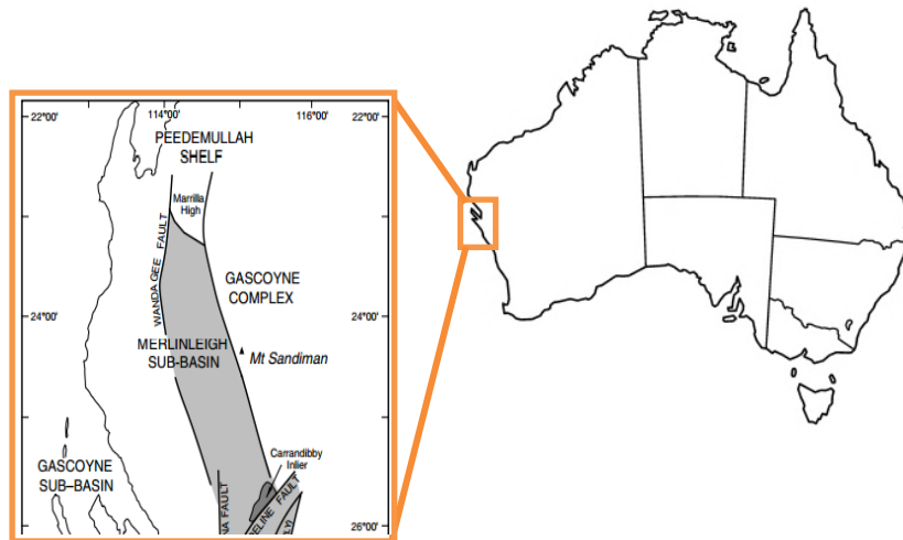
Figure 1 - Location of the Merlinleigh Sub-basin, Western Australia
