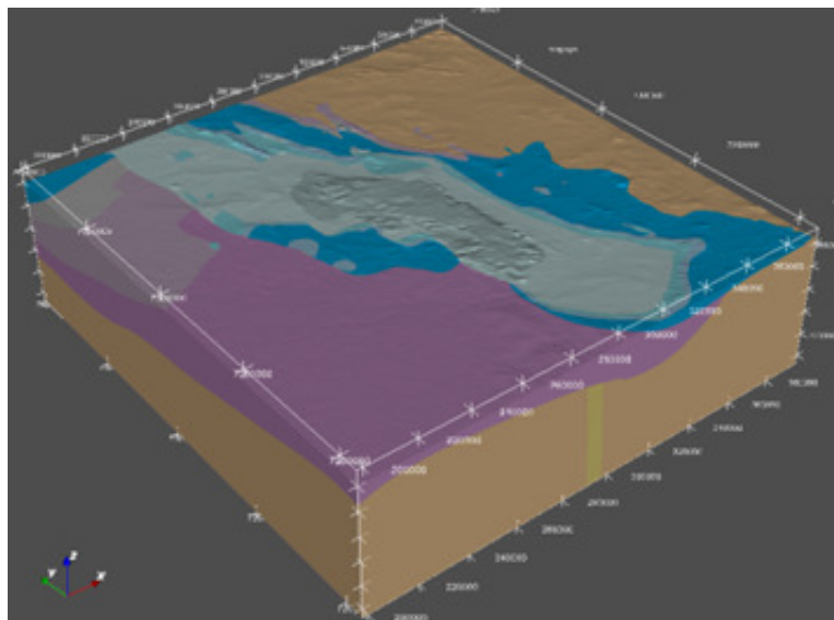
Figure 10 - The most-probable geological model of the Merlinleigh Sub-basin from the post-inversion statistical distillation of all possible models. A key outcome of the case study; this is the culmination of all applied processing and interpretation workflows.
