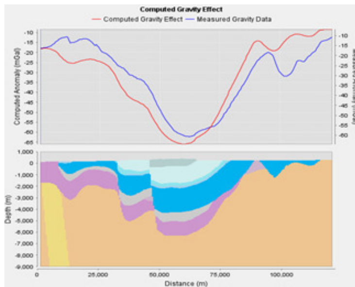
Figure 8 - Profile modelling (2D forward modelling) through the Merlinleigh Sub-basin 3D geology model, performed for the purpose of refining the model, prior to 3D forward modelling, and full geophysical inversion. (A close model fitting all independent data sets is the best starting point for inversion.)
