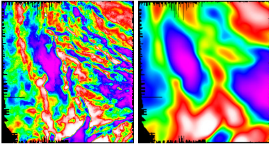
Figure 5 - Grids of the Merlinleigh Sub-basin gravity data. Left: residual signals, Right: regional signal.
