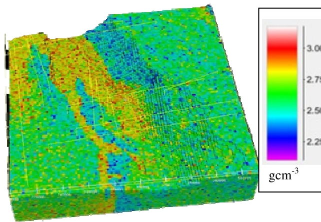
Figure 7 - Resulting block model of density for the Merlinleigh Sub-basin, after rock property optimisation. A key finding was the indication of a high density body (around 2.8 \text{ gcm}^{-3} ) along the Wandagee fault, located in the basement zone.
