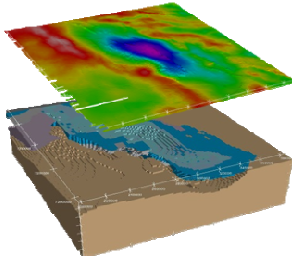
Figure 9 - Upper: Gravity anomaly grid. Lower: Discretised starting geology model (block model or “lithology voxel”) of the Merlinleigh Sub-basin prior to inversion, with the basement visible.
