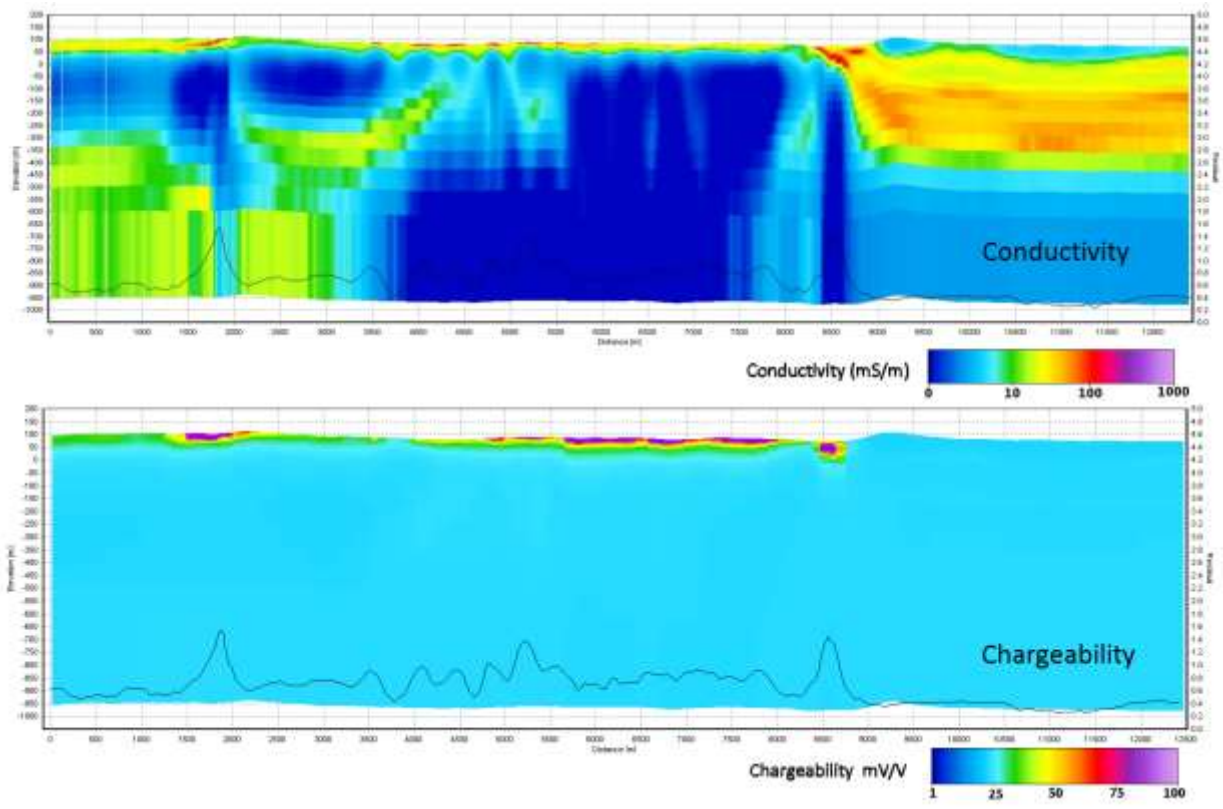
Figure 7: AarhusInv 1D inversion results for Line 10440 derived by solving for resistivity (conductivity), chargeability, frequency and a time constant together. Only the results for conductivity and chargeability with associated misfit (black line in both plots), are shown. The inversion indicates that there are chargeable regolith (?) layers in the near surface, which are also conductive. The conductivity model is similar to that shown in Figure 6A, including what could be interpreted as folded conductors (between 4000 and 6000m). Only the deeper conductive layer in the middle of the section is missing. The data are well fitted throughout the section (particularly when compared with the data misfit in Figure 6A – grey line).
