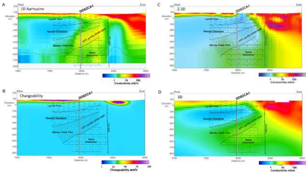
Figure 8: Enlarged section of Line 10440 (between 7000 and 9000m in Figure 7), for the area adjacent to the Emu Fault. The 1D inversion results (A) define a conductor associated with the HYC pyritic shale unit intersected in drillhole DD82CA1. A broad conductive zone is defined for that part of the stratigraphy and deeper in the 3D results (D), whereas the 2.5D inversion appears to define a more conductive zone at greater depth (C). A chargeable response is only defined in the near surface regolith (B).
